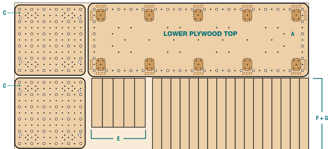
PLYWOOD LAYOUT 2
