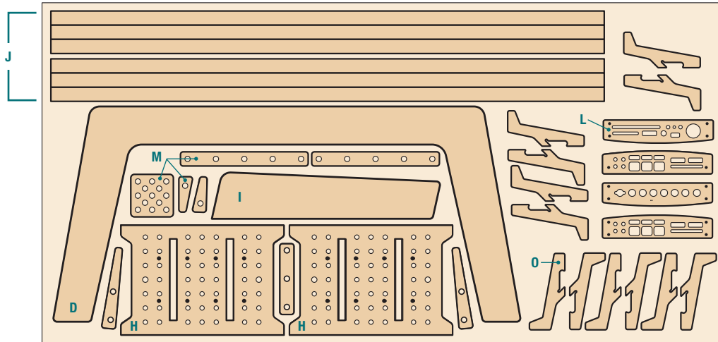
PLYWOOD LAYOUT 3
