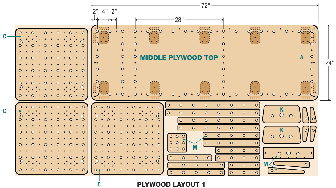
PLYWOOD LAYOUT 1
